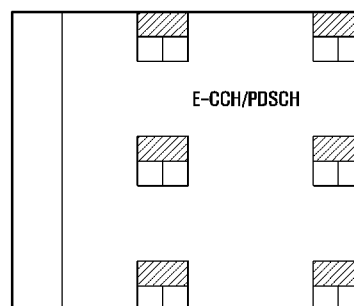
DMRS port configuration for Agg. Lv. 4&amp;8
