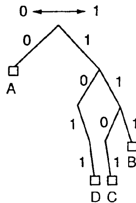
DECODING TREE IN BACKWARD DIRECTION
