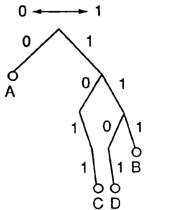
DECODING TREE IN FORWARD DIRECTION
