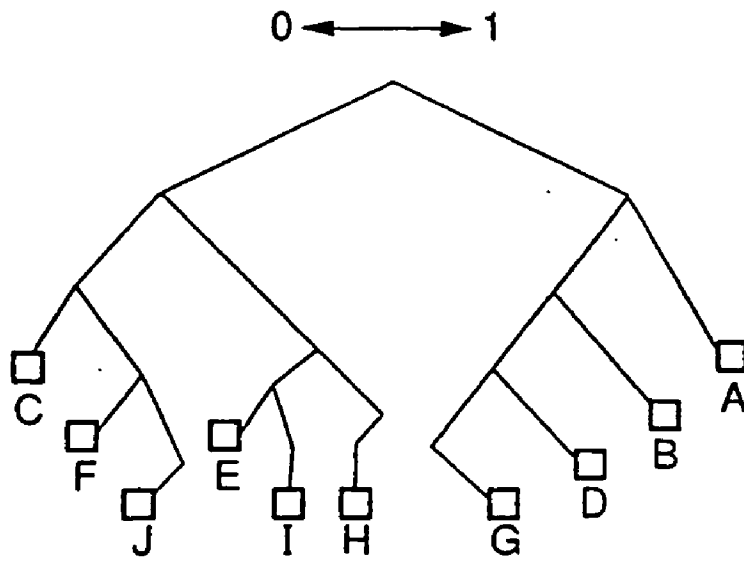
DECODING TREE IN FORWARD DIRECTION
