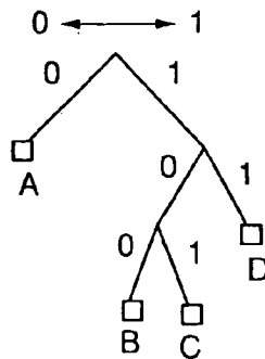
DECODING TREE IN FORWARD DIRECTION
