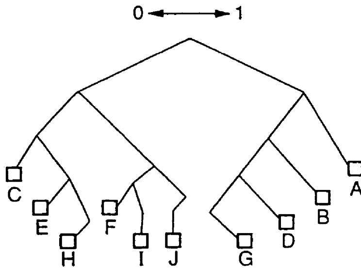
DECODING TREE IN BACKWARD DIRECTION
