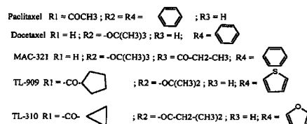
Chemical Structure of Taxanes
