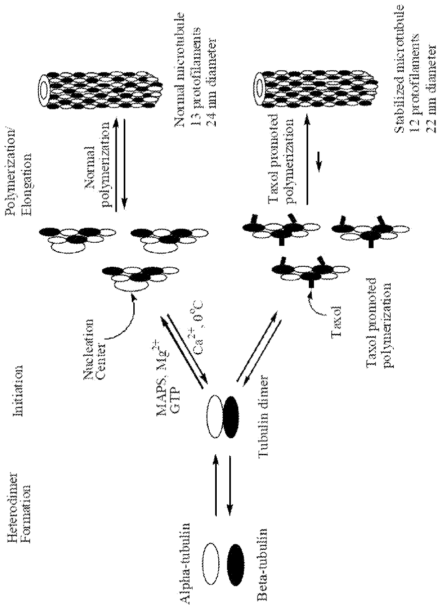
FIG. 2 Tubulin-microtubule dynamics (Kingston 2001)
