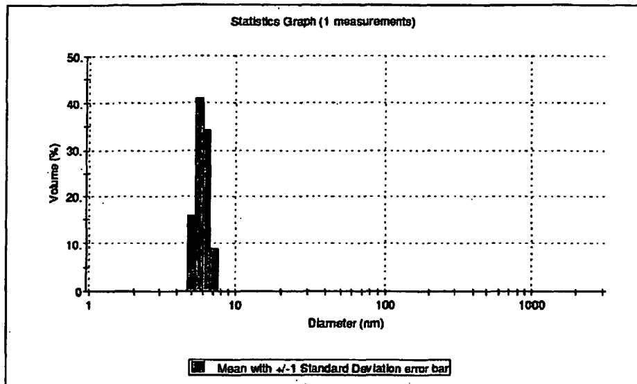
Figure 5. The Particle Size Analysis of 4% Albumin.
