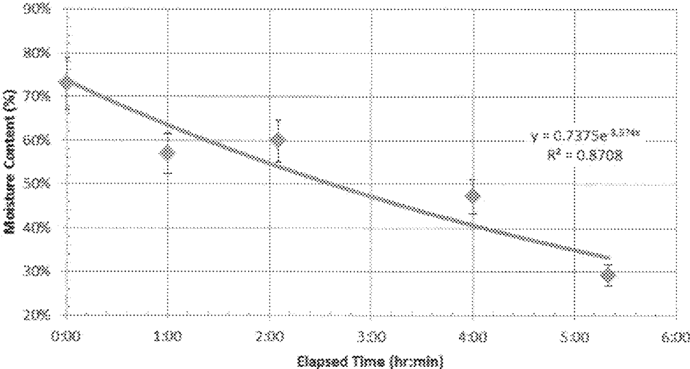
Figure 9. Drying of Food Waste in Prototype
