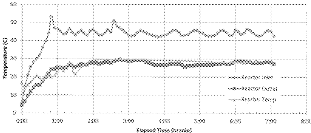
Figure 10. Temperatures during Food Waste Drying in Prototype
