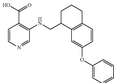
3-[(7-phenoxy-1,2,3,4-tetrahydronaphthalen-1-yl)methyl]amino]pyridine-4-carboxylic acid
