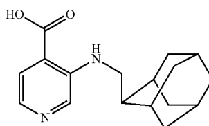
3-[(adamantan-2-ylmethyl)amino]pyridine-4-carboxylic acid
