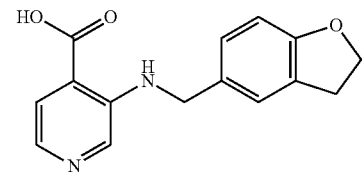
3-[2,3-dihydro-1-benzofuran-5-ylmethyl]amino]pyridine-4-carboxylic acid
