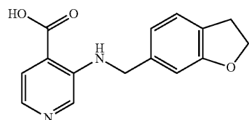
3-[2,3-dihydro-1-benzofuran-6-ylmethyl]amino]pyridine-4-carboxylic acid
