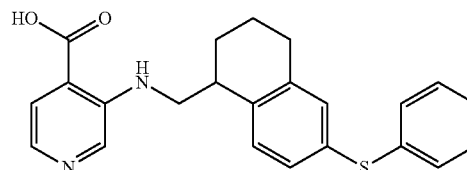
3-[(6-(phenylsulfanyl)-1,2,3,4-tetrahydronaphthalen-1-yl)methyl]amino]pyridine-4-carboxylic acid
