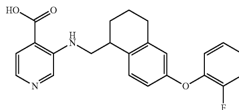
3-({[6-(2-fluorophenoxy)-1,2,3,4-tetrahydronaphthalen-1-yl]methyl}amino)pyridine-4-carboxylic acid
