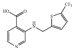
5-[[5-(5-(trifluoromethyl)thiophen-2-yl)methyl]amino]pyridine-4-carboxylic acid
