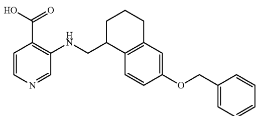
3-[(6-benzyloxy-1,2,3,4-tetrahydronaphthalen-1-yl)methyl]amino]pyridine-4-carboxylic acid
