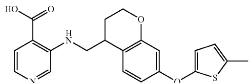
3-[(6-[(5-methylthiophen-2-yl)oxy]-1,2,3,4-tetrahydronaphthalen-1-yl)methyl]amino]pyridine-4-carboxylic acid
