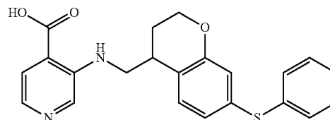
3-[(7-(phenylsulfanyl)-3,4-dihydro-2H-1-benzopyran-4-yl)methyl]amino]pyridine-4-carboxylic acid
