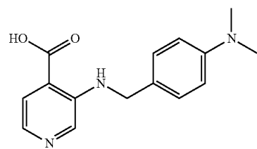
3-{[4-(dimethylamino)benzyl]amino}pyridine-4-carboxylic acid
