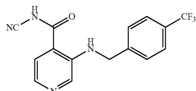
N-cyano-3-(4-(trifluoromethyl)benzylamino)isonicotinamide
