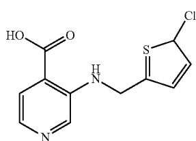
5-[[5-(5-chlorothiophen-2-yl)methyl]amino]pyridine-4-carboxylic acid
