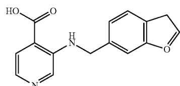
3-[(1-benzofuran-6-ylmethyl)amino]pyridine-4-carboxylic acid
