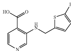
5-[[5-(5-fluorothiophen-2-yl)methyl]amino]pyridine-4-carboxylic acid
