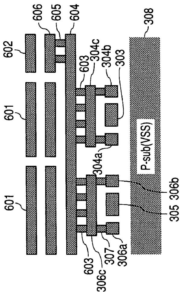
FIG. 6B SECTIONAL VIEW
