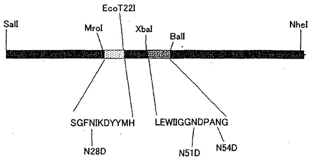
B HEAVY CHAIN VARIABLE REGION OF ANTI-HUMAN TF ANTIBODY (425 bp)
