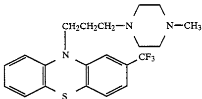
trimeprazine: 10-[3-(dimethylamino)-2-methylpropyl]phenothiazine
