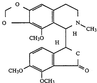
noscapine: 6,7-dimethoxy-3-(5,6,7,8-tetrahydro-4-methoxy-6-methyl-1,3-dioxolo[4,5-g]isoquinolin-5-yl)-1(3H)-isobenzofuranone
