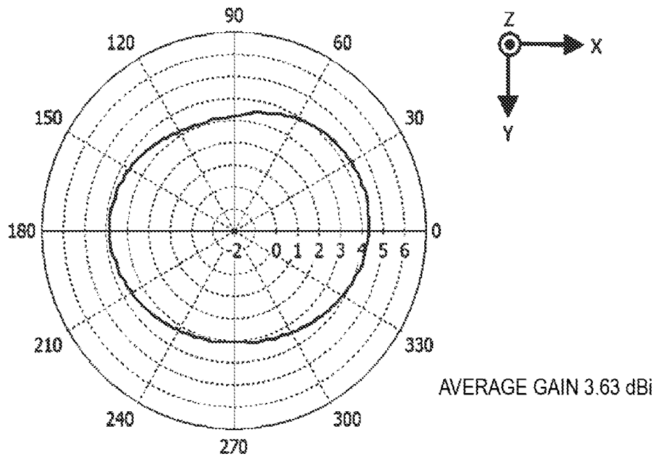
GAIN [dBi] IN X-Y PLANE (HORIZONTAL PLANE) OF VERTICAL POLARIZED WAVE AT 5850 MHz
