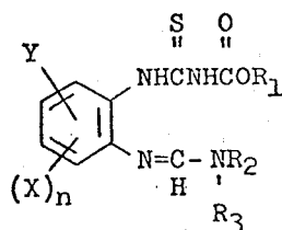
(Formula III)
