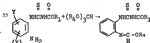
(Formula II)
