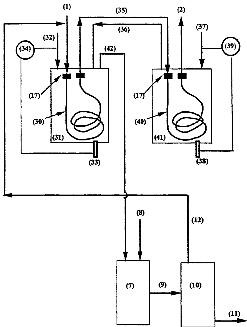
Figure 6 - Two stage aromatic amine recovery process
