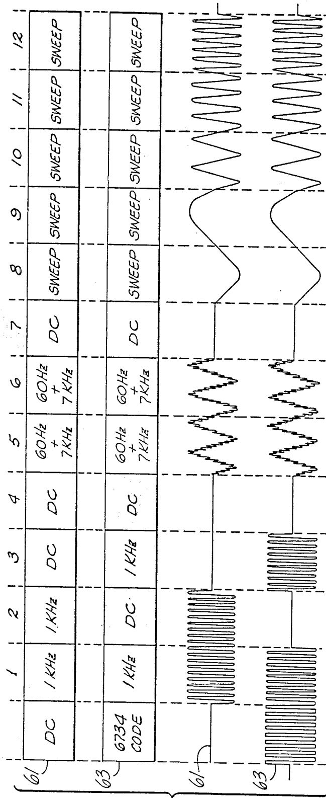
FIG. 6 AUDIO TEST TONE PLACEMENT.
