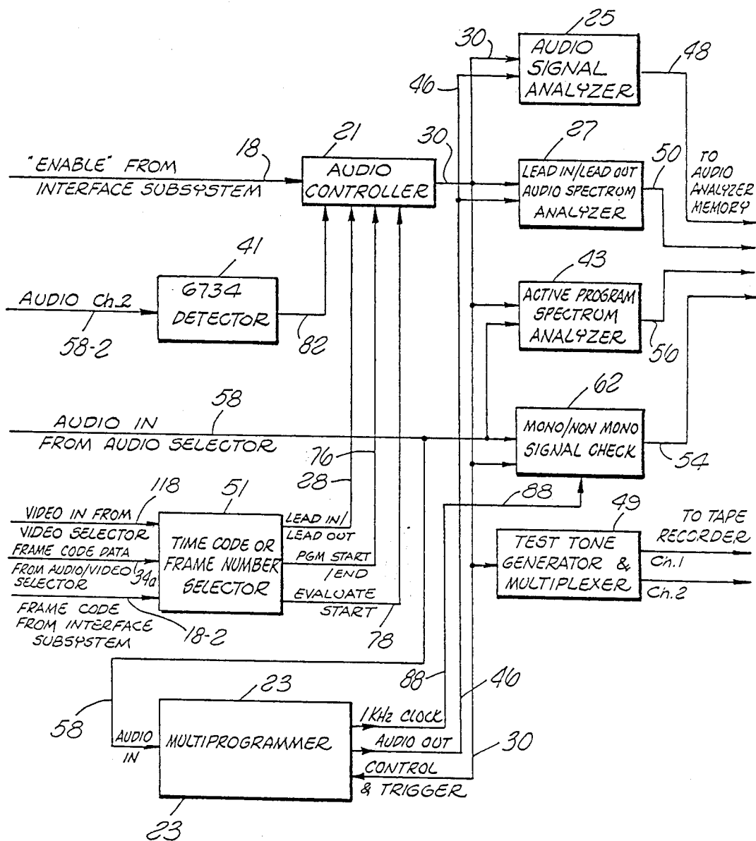
FIG. 4 - AUDIO TEST SUBSYSTEM
