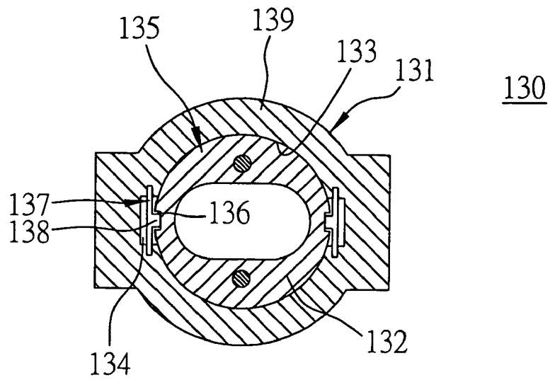
FIG. 10 (PRIOR ART)
