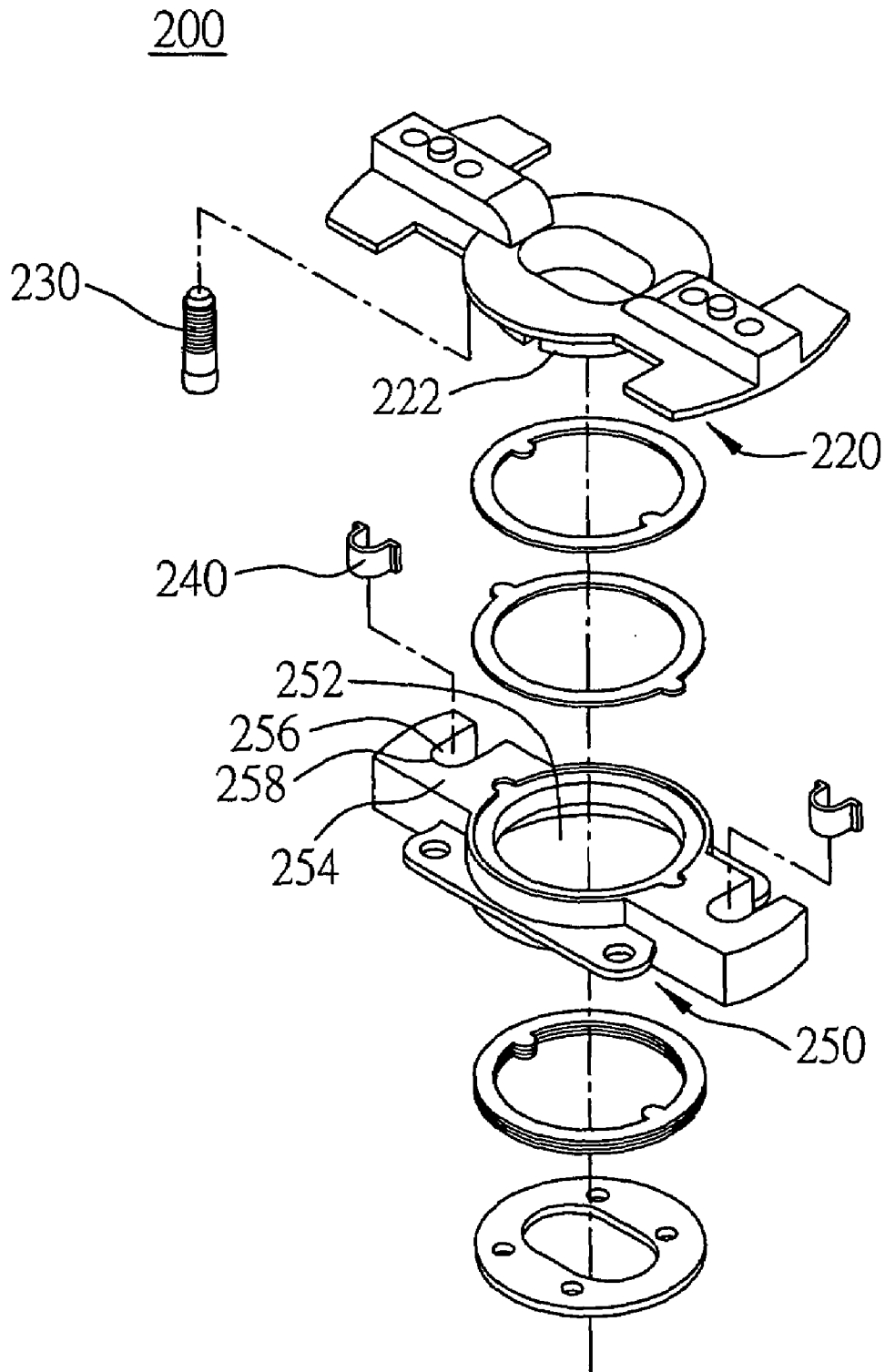
FIG. 12 (PRIOR ART)
