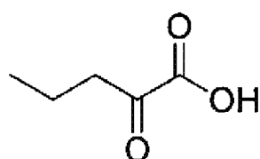
2-oxopentanoic acid
