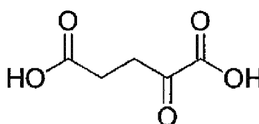
2-oxoglutaric acid
