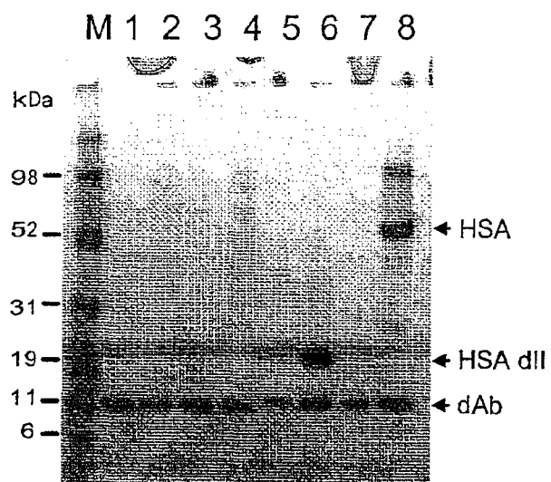
Figure 22. Example of an immunoprecipitation showing that a HSA binding dAb binds full length HSA (lane 8) and HSA domain II (lane 6), but does not bind HSA domains I and III (lanes 5 and 7). A non-HSA binding dAb does not pull down either full length HSA or HSA domains I, II, or III (lanes 1-4)
