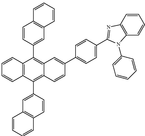
&lt;Compound 102&gt;
