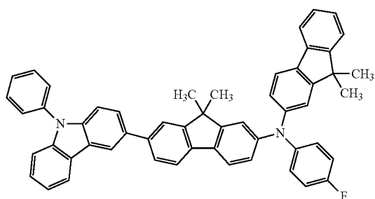
&lt;Compound 3&gt;
