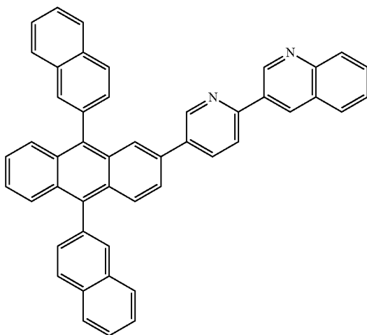
&lt;Compound 102&gt;
