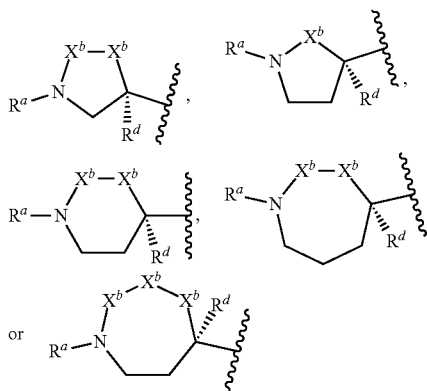
[Chemical formula 37]
