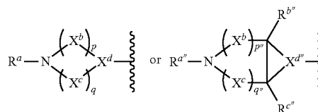
[Chemical formula 31]
