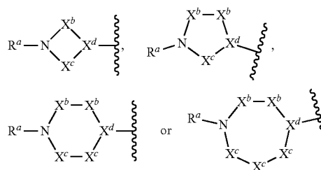
[Chemical formula 33]
