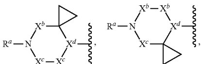
[Chemical formula 28]
