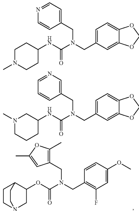
[Chemical formula 13]
