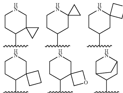
[Chemical formula 24]
