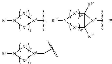
[Chemical formula 17]
