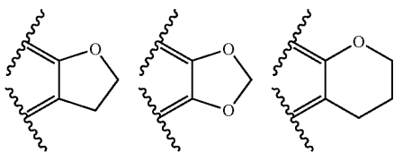
[Chemical formula 27]
