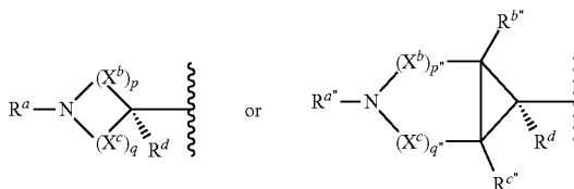
[Chemical formula 34]
