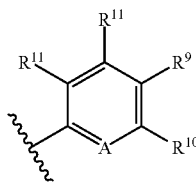
[Chemical formula 11]
