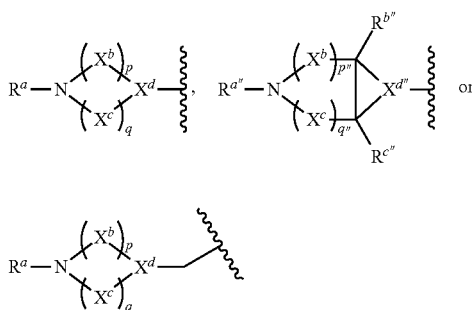
[Chemical formula 30]
