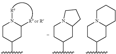
[Chemical formula 26]
