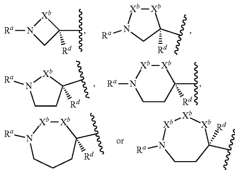
[Chemical formula 36]
