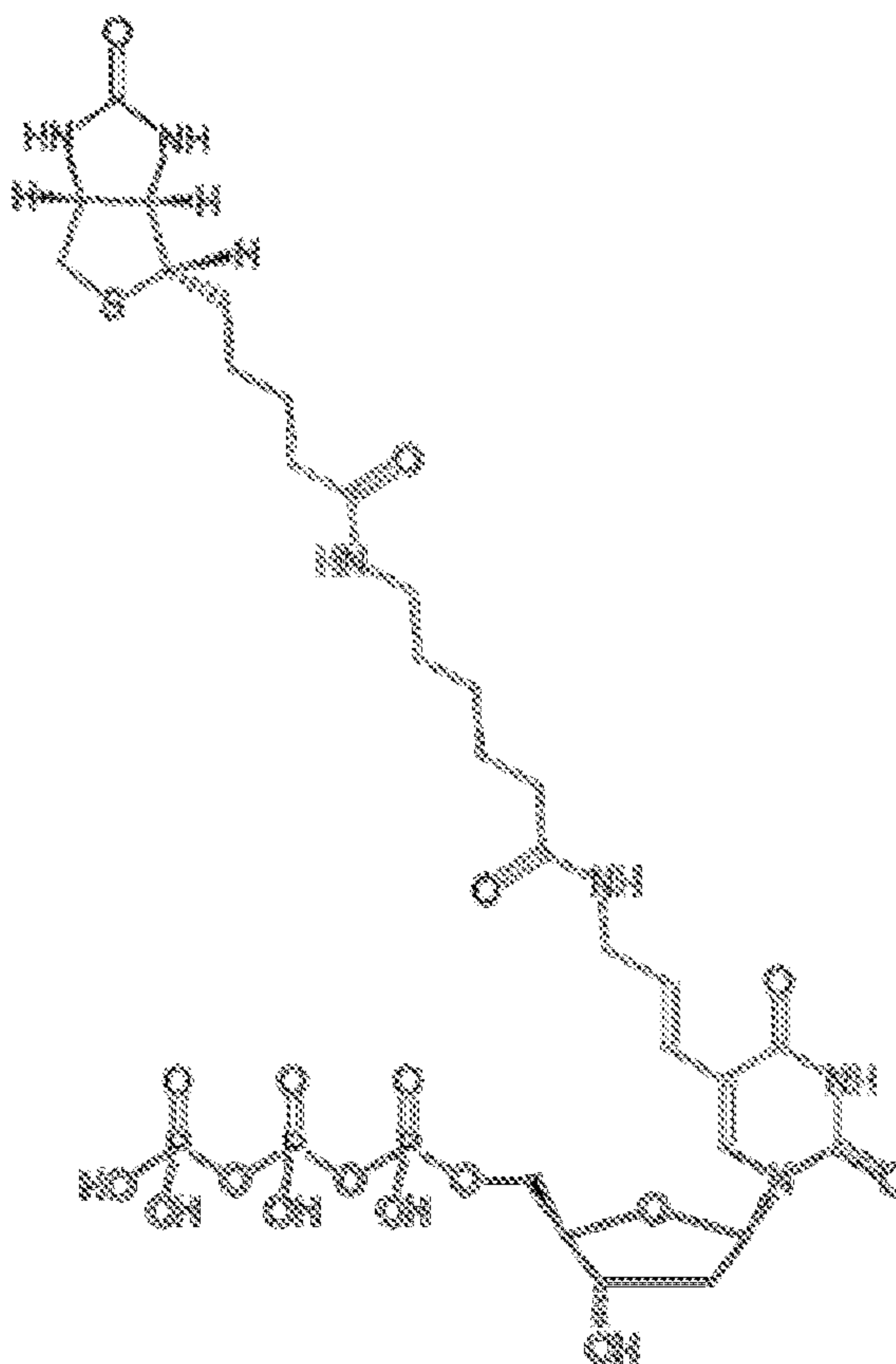
Biotin-11-dUTP
