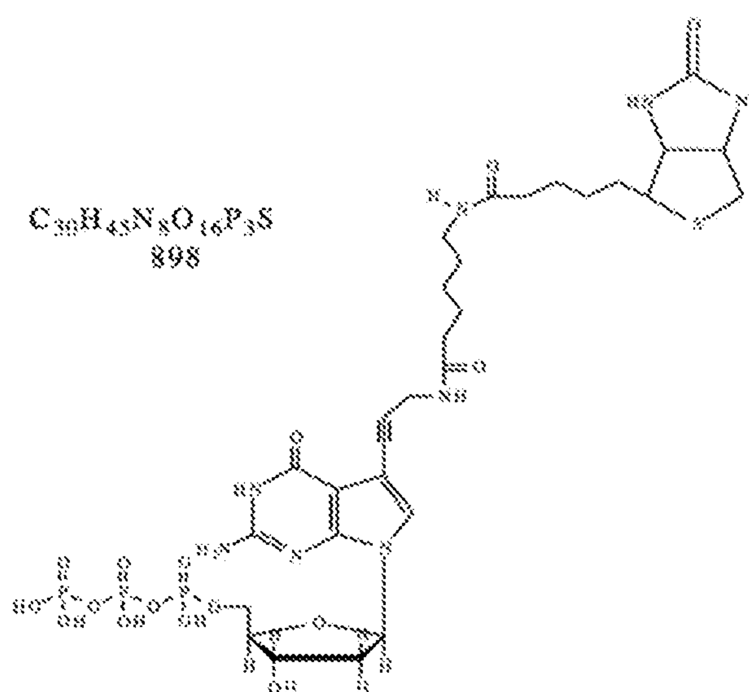
Biotin-11-dGTP
