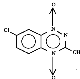
11 7-chloro-3-hydroxy-1,2,4-benzotriazine-1,4-dioxide
