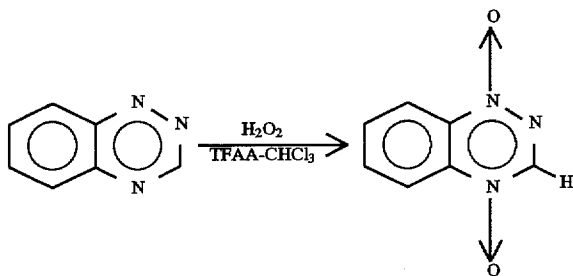
8 1,2,4-benzotriazine
