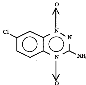
12 7-chloro-3-amino-1,2,4-benzotriazine-1,4-dioxide
