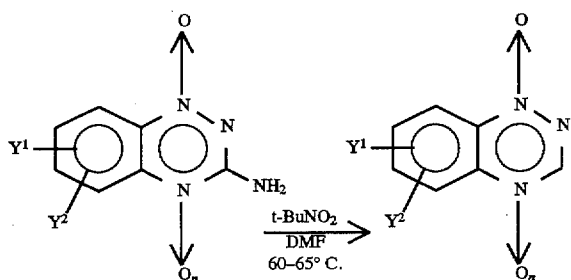
Scheme V
