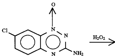
10 7-chloro-3-amino-1,2,4-benzotriazine-1-oxide
