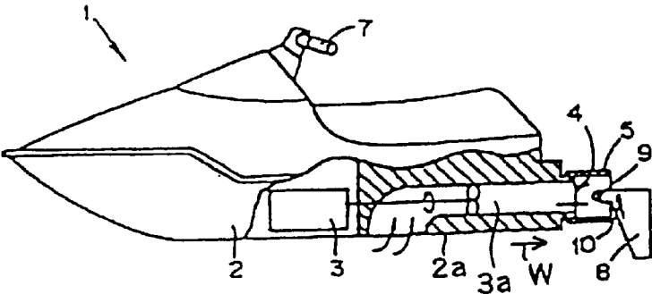
FIG. 5 (a) BACKGROUND ART
