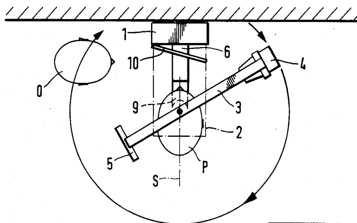
Fig. 1 PRIOR ART
