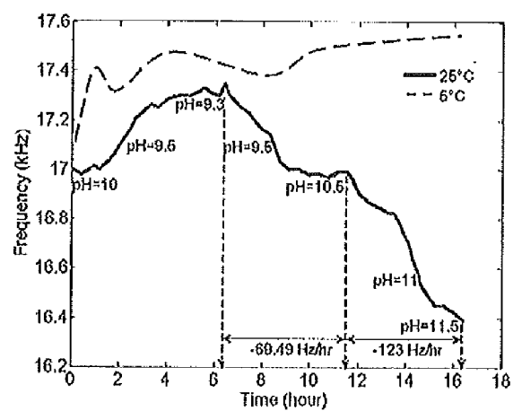
Figure 31 The modulated frequencies transduced from the fish filets with the wireless pH sensor tag wrapped in the package.
