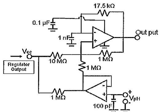
Figure 20 The relaxation oscillator design in the transponder.
