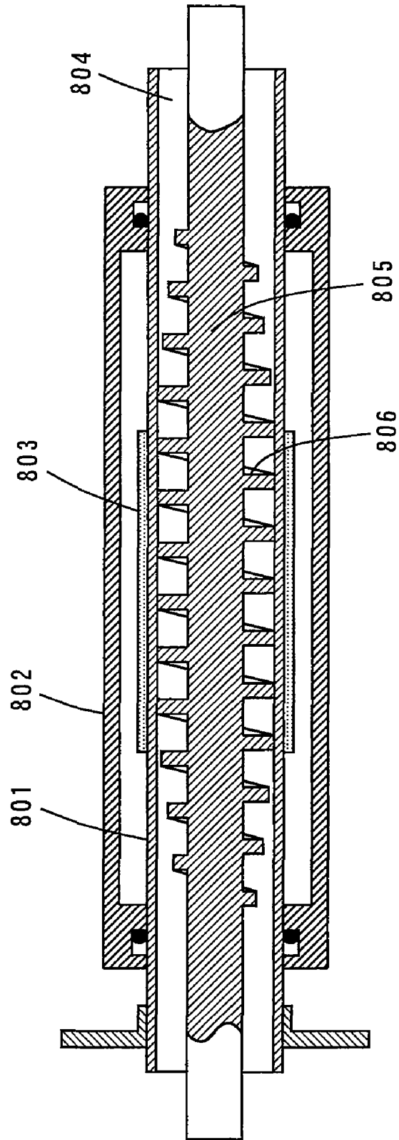
FIG. 48 PRIOR ART
