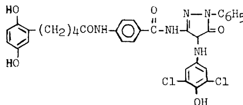
Compound IV
