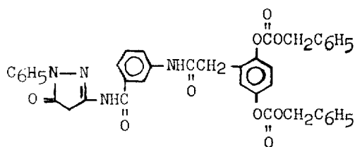
Intermediate 3-A
