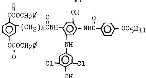
Intermediate 7-A
