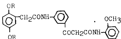
Compound 5-A
