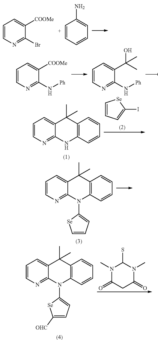
[Reaction Scheme 1]
