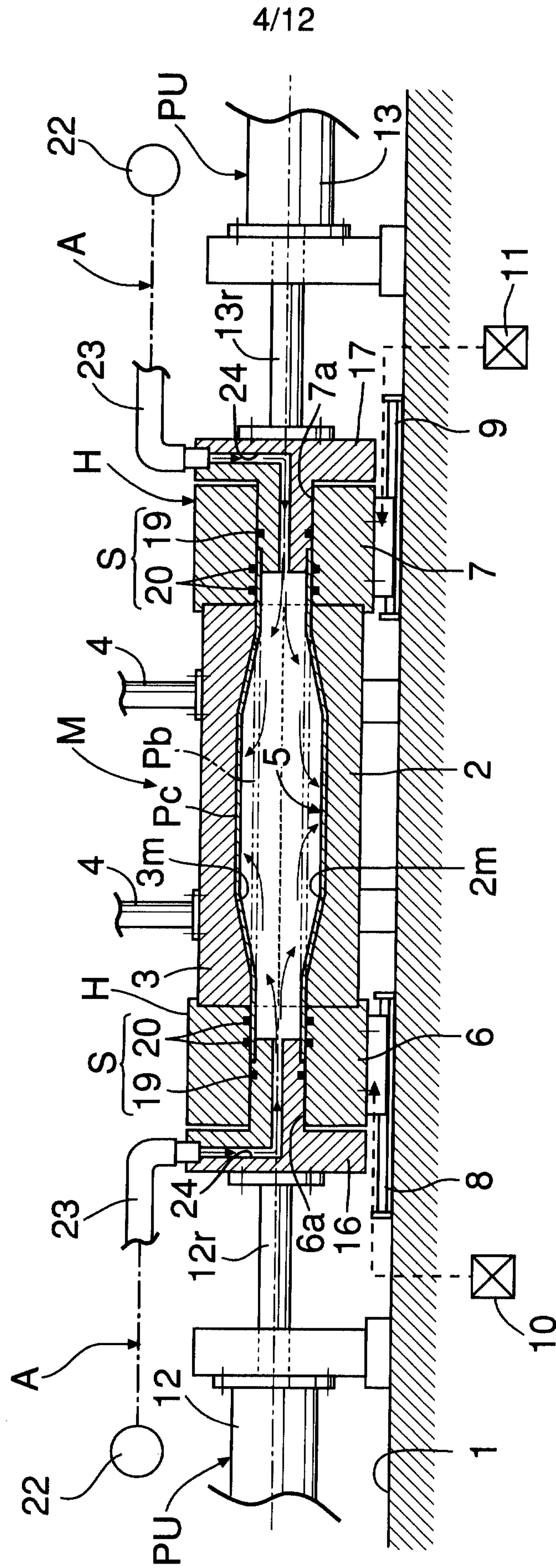
FIG.4 TUBE-EXPANDING (BULGE-FORMING) STEP
