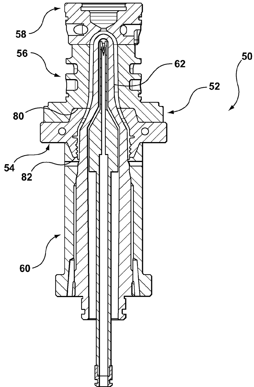
FIG. 1 (PRIOR ART)
