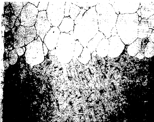
FIG. 4 Stellite Alloy No. 1 Cladding (top) - steel tube I.D. interface at 400X. Etchant: Picral
