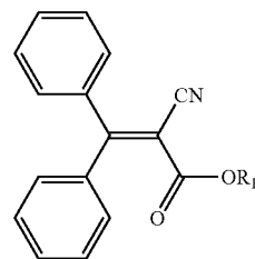
cyanoacrylate
