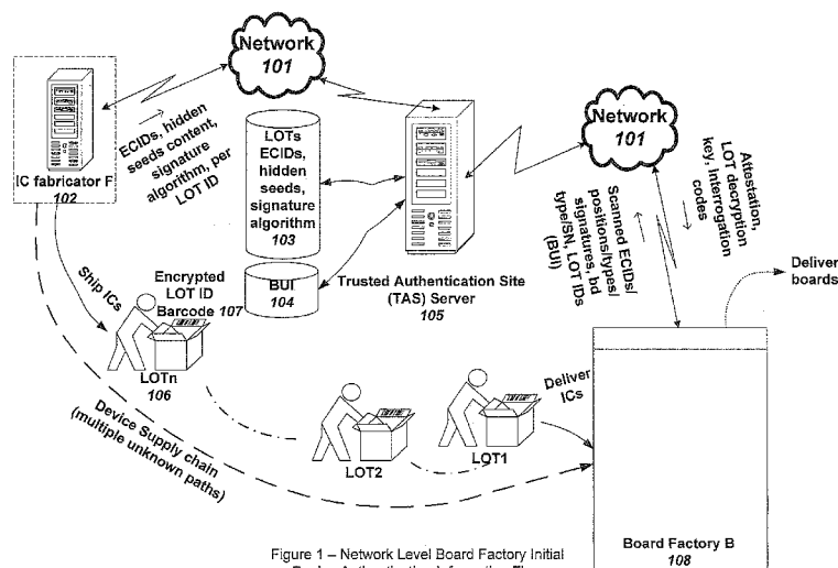
Figure 1 - Network Level Board Factory Initial Device Authentication Information Flow
