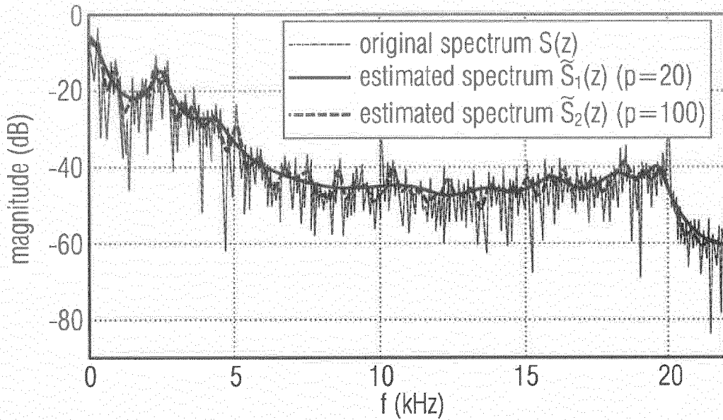
Original spectrum of a speech signal segment of 1024 samples and two of its approximations, the first (black curve) with a lower and the second (dashed curve) with higher prediction order.
