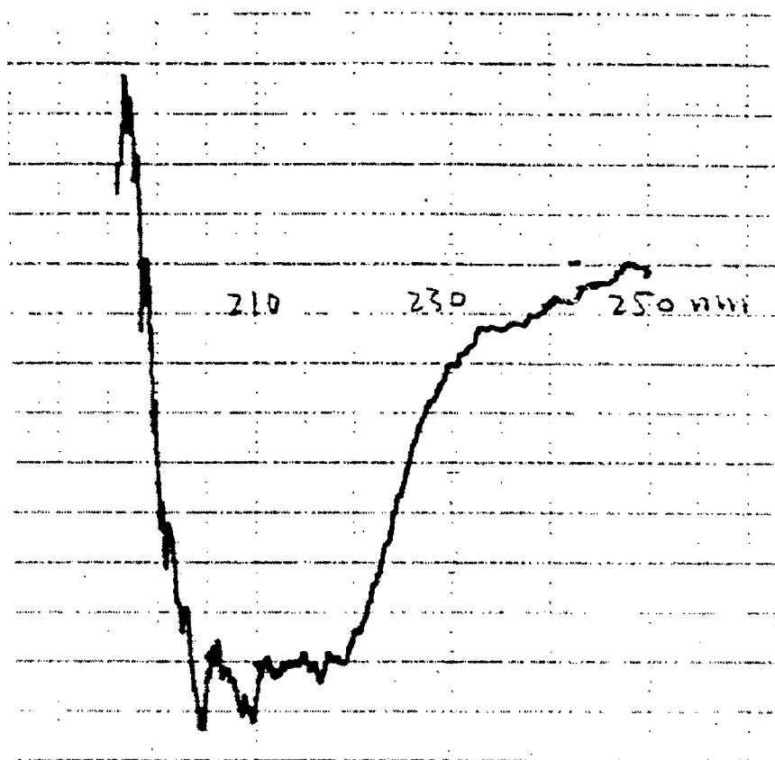
Fig 6-D Circular Dichroism spectrum of rSIFN-co
