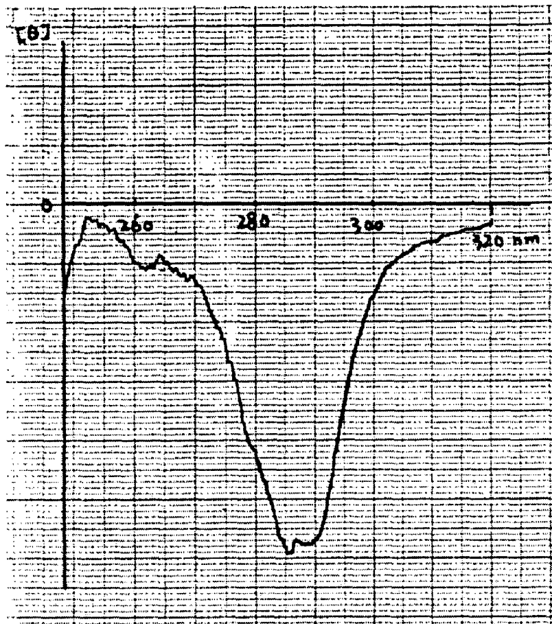
Fig 6-C Circular Dichroism spectrum of rSIFN-co
