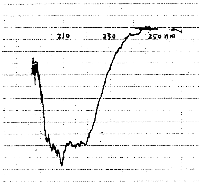
Fig 6-A Circular Dichroism spectrum of Infergen
