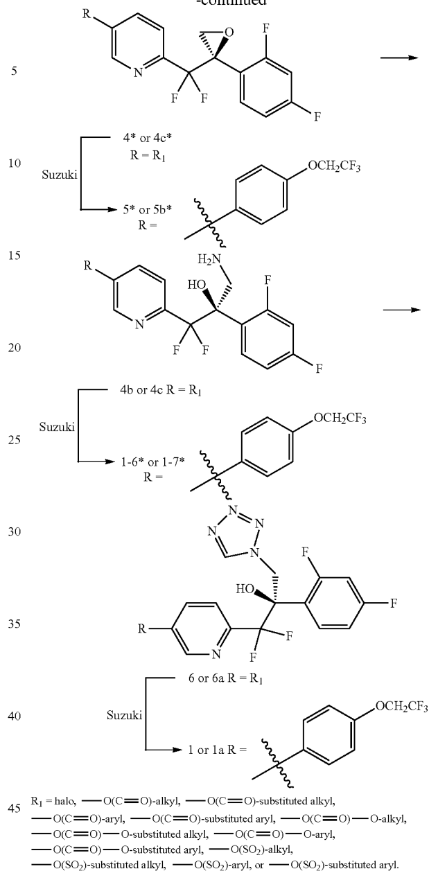
Scheme 3. Synthesis of 1 via Asymmetric Dihydroxylation Method
