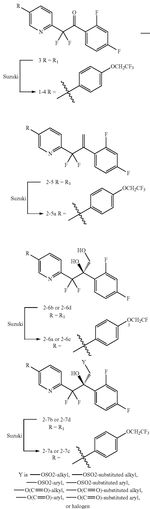
Scheme 3. Synthesis of 1 via Asymmetric Dihydroxylation Method
