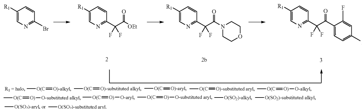
Scheme 2. Synthesis of ketone 3
