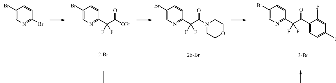
Scheme 1. Synthesis of ketone 3-Br
