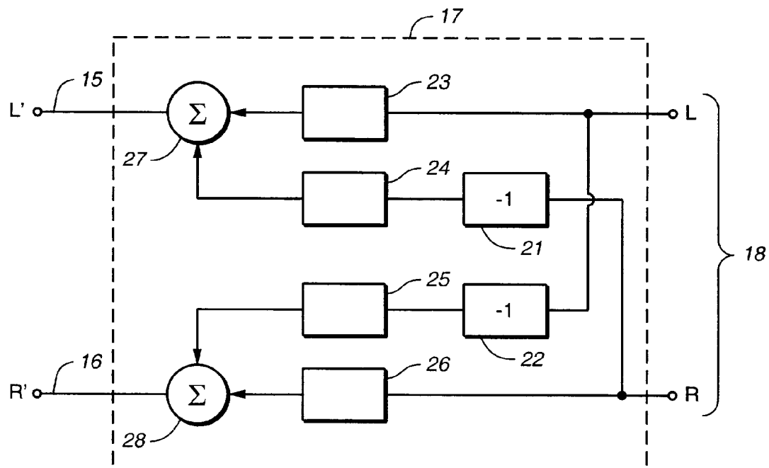
FIG. 2 (PRIOR ART)
