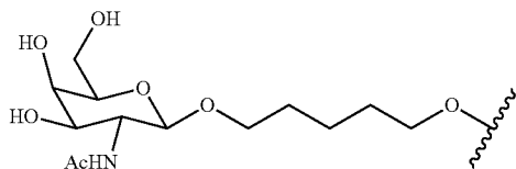
Example 111: Synthesis of Oligonucleotides Comprising a GalNAc 2-31 or GalNAc 2-32 Conjugate
