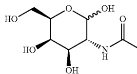
2-(Acetylamino)-2-deoxy-D-galactopyranose
