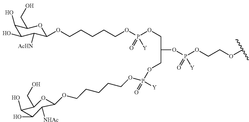
Example 112: Modified Oligonucleotides Comprising a GalNAc 1 Conjugate
