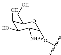
2-(Acetylamino)-2-deoxy-α-D-galactopyranose
