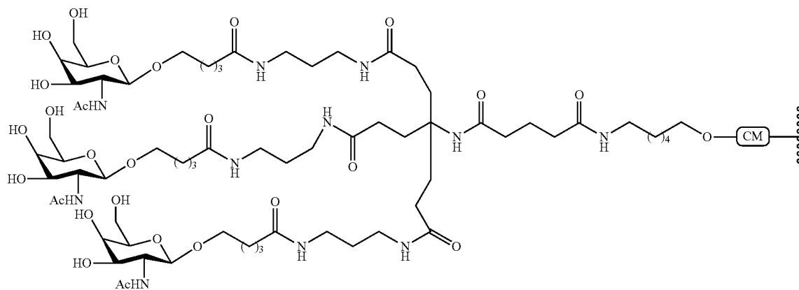
Example 69: Preparation of Oligomeric Compound 201 Comprising GalNAc 3 -18
