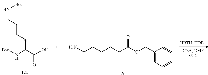
Example 104: Synthesis of Oligonucleotides Comprising a 5'-GalNAc 2 Conjugate
