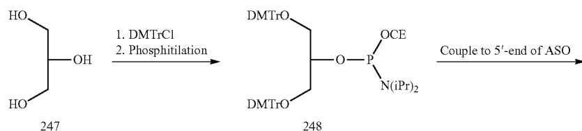
Example 111: Synthesis of Oligonucleotides Comprising a GalNAc 2-31 or GalNAc 2-32 Conjugate
