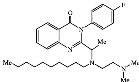
2-[1-[Decyl-(2-dimethylamino-ethyl)-amino]-ethyl]-3-(4-fluoro-phenyl)-3H-quinazolin-4-one (Compound 2.3)
