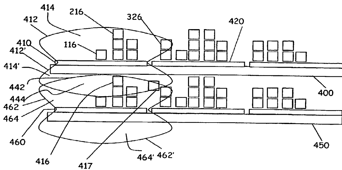
FIG. 4 Front Elevation View
