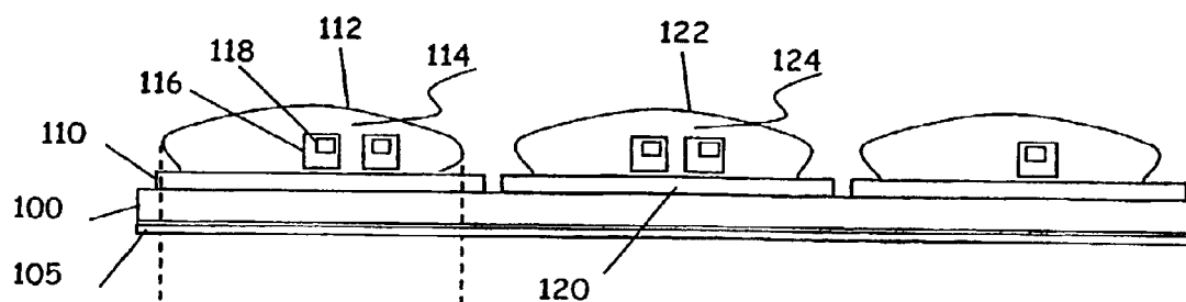
FIG. 1A Front Elevation View
