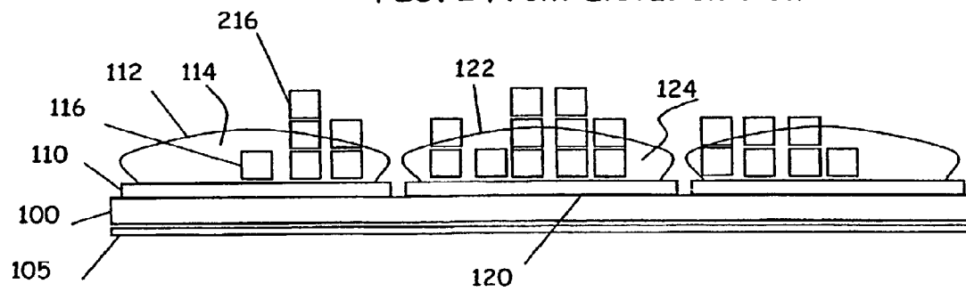
FIG. 2 Front Elevation View
