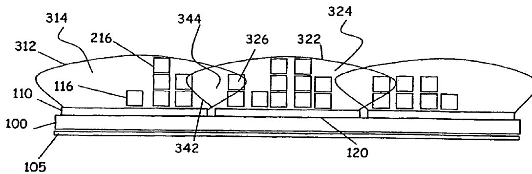
FIG. 3A Front Elevation View
