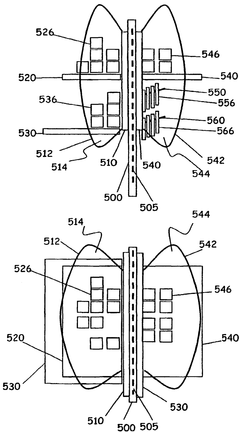
FIG. 5A Side Elevation View
