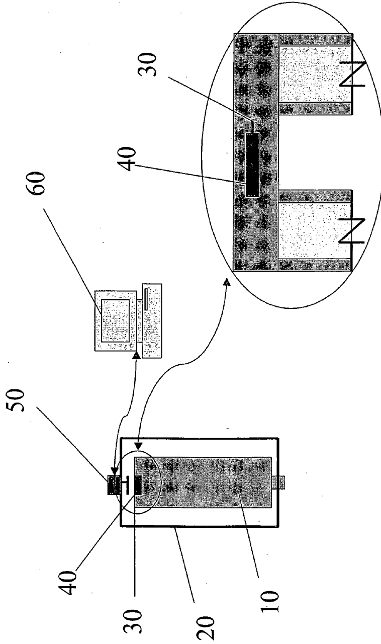
Figure 1: Temperature Probe / RFID Communication Device within Filter Endcap
