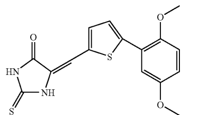
Compound E8
