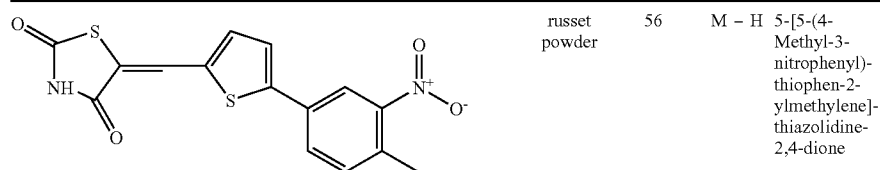
Compound F12
