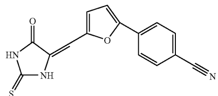
Compound E5
