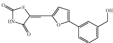
Compound F3
