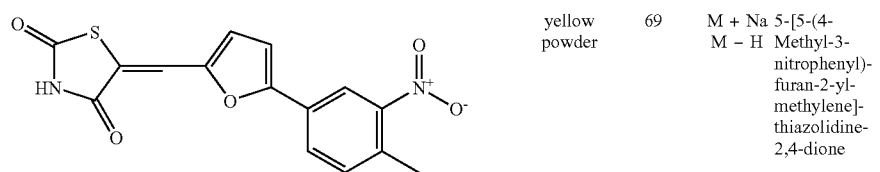
Compound F6
