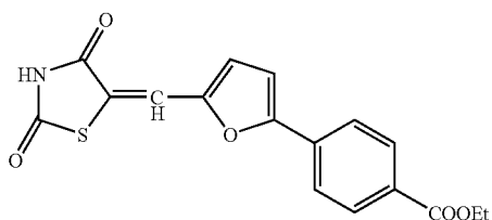
Compound 3: 5-({5-[3,5-bis(Trifluoromethyl)phenyl]-2-furyl}methylene)-1,3-thiazolidine-2,4-dione
