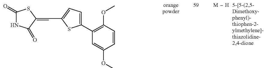
Compound F10
