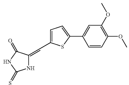
Compound E7
