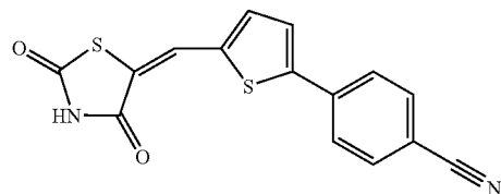
Compound F13
