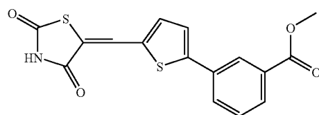
Compound F14
