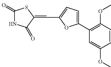
Compound F4
