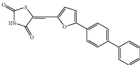
Compound F2
