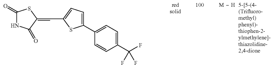
Compound F11
