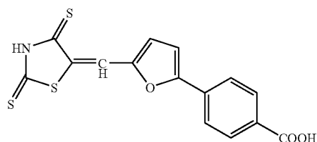
Compound 8: Disodium salt of 4-{5-[(2,4-disulpho-1,3-thiazolidin-5-ylidene)methyl]-2-furyl}benzoic acid (isomer Z)
