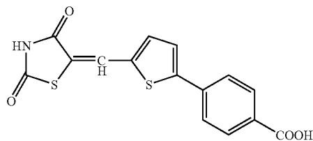
Compound 6: 4-{5-[(2-Sulpho-4-oxo-1,3-thiazolidin-5-ylidene)methyl]-2-furyl}benzoic acid
