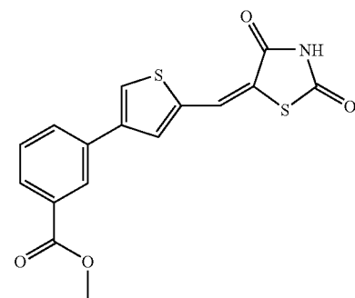
Compound F16
