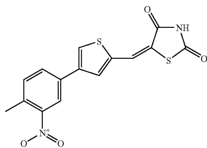
Compound F15
