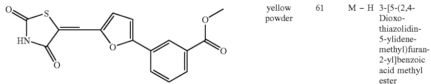
Compound F8
