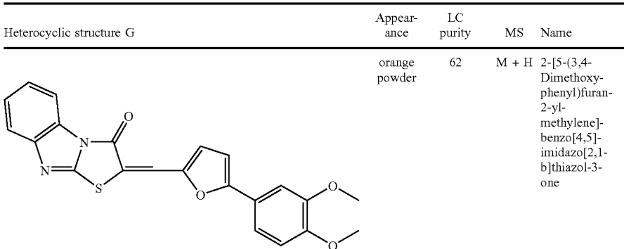
Compound G1
