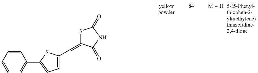
Compound F18
