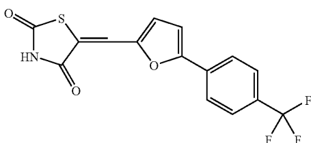
Compound F5
