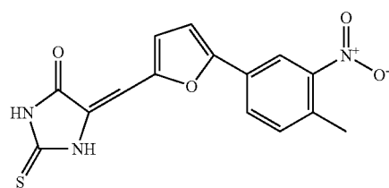
Compound E4
