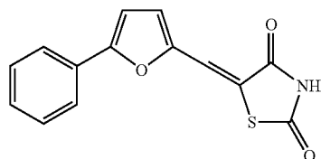
Compound F17
