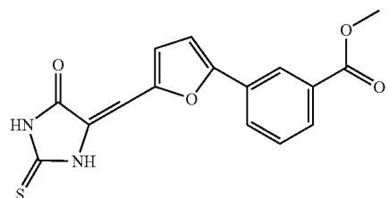
Compound E6
