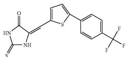
Compound E9
