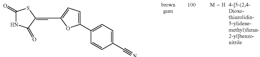
Compound F7
