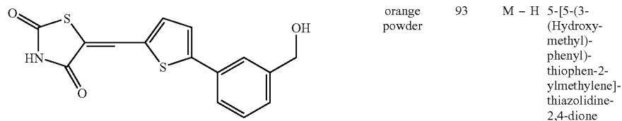
Compound F9
