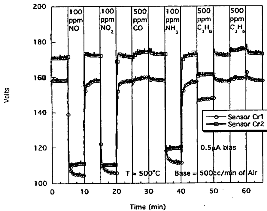
Comparison of two TapeCasted NO x sensors
