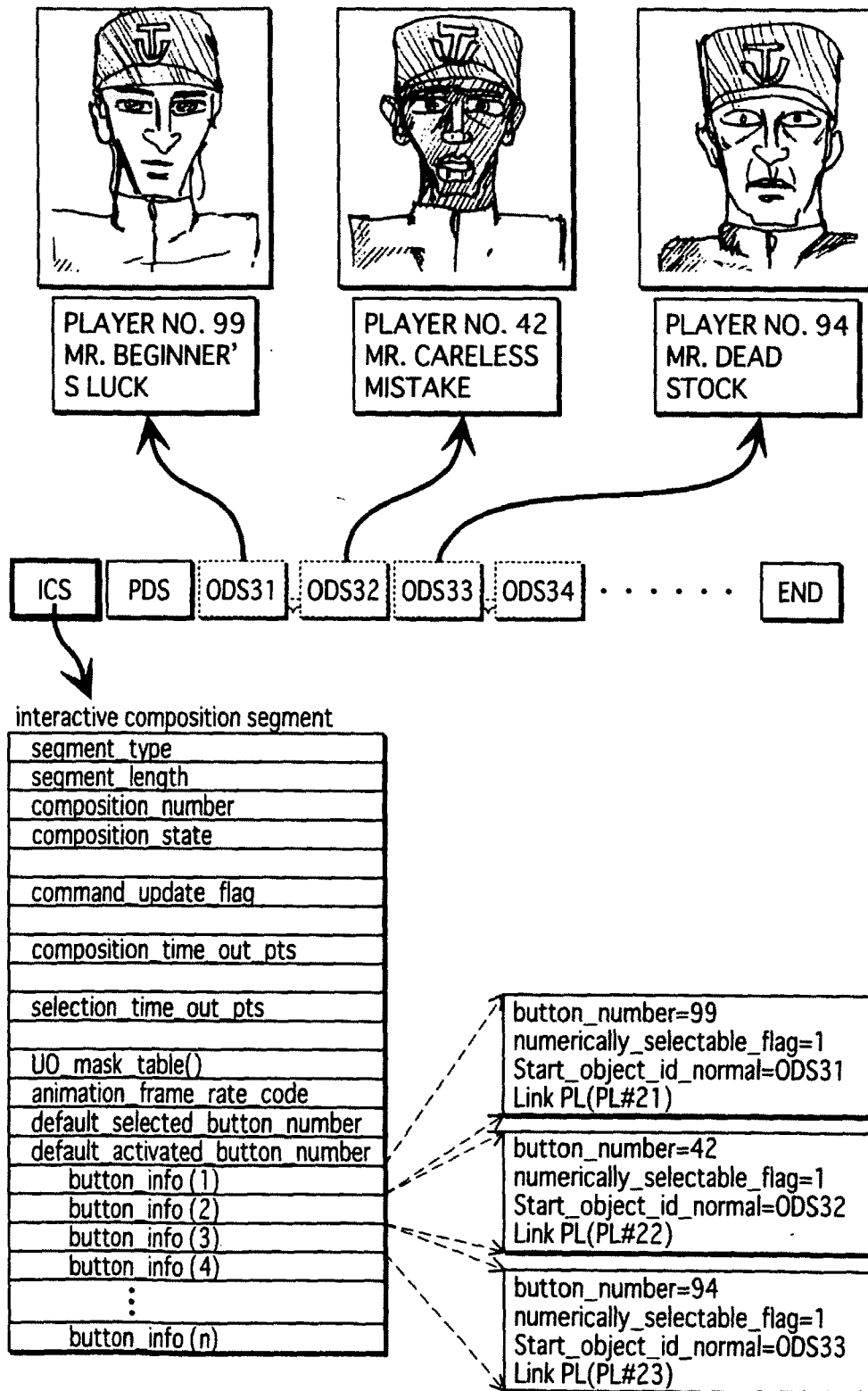
FIG.18 PLAYERS LIST
