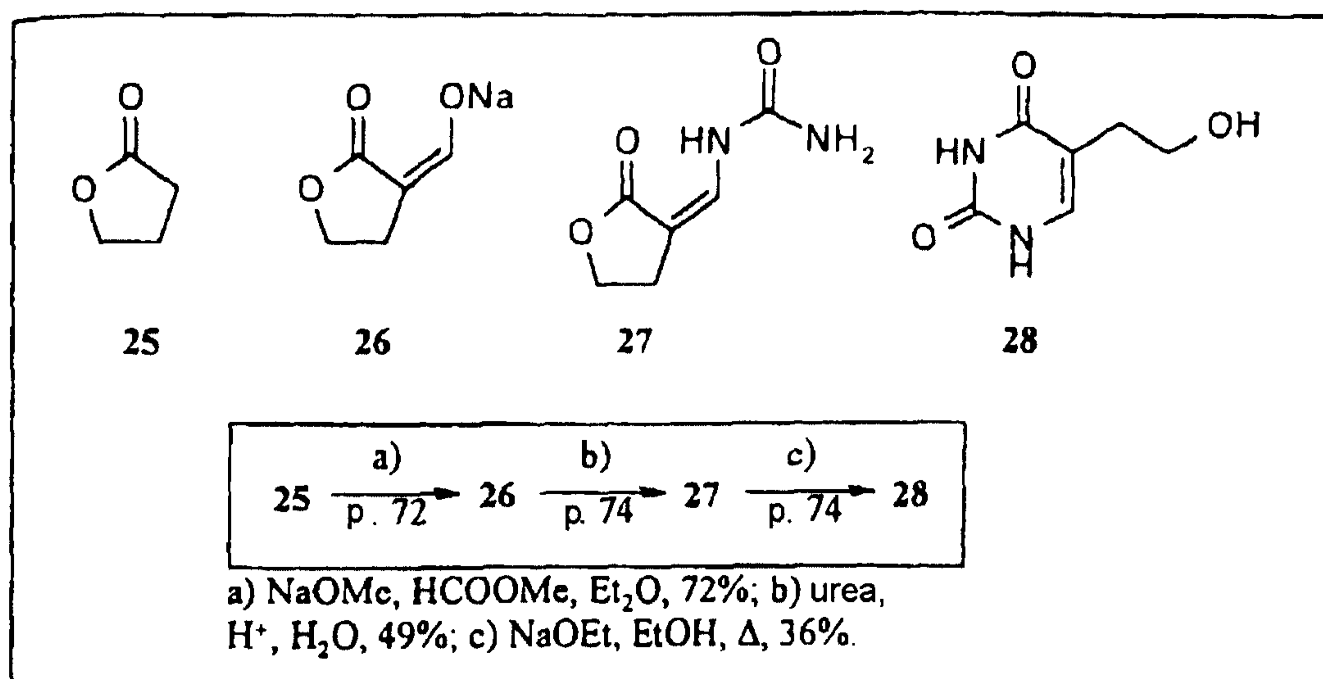
Scheme 4: Synthesis of hydroxyethyluracil 28.
