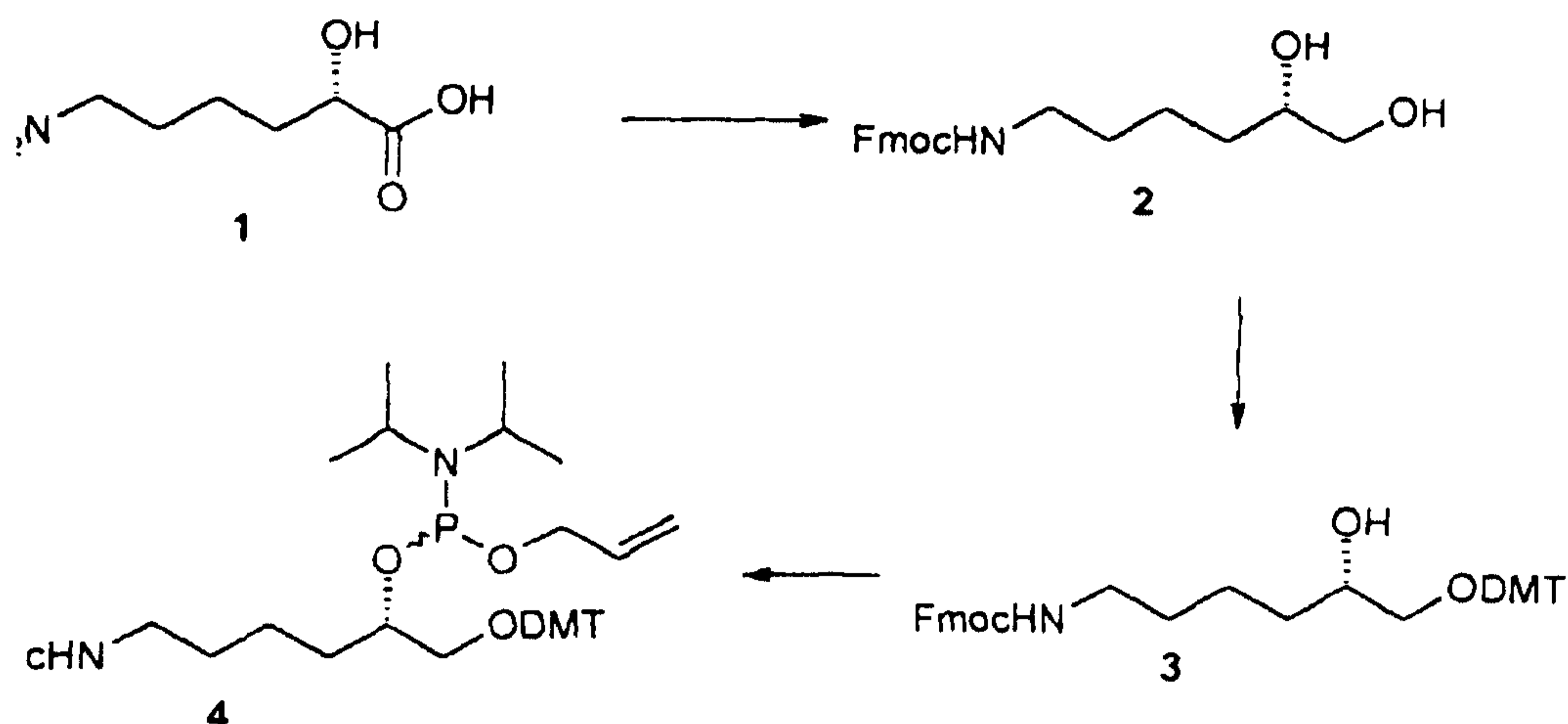
Scheme 7: Synthesis of the lysine linker
