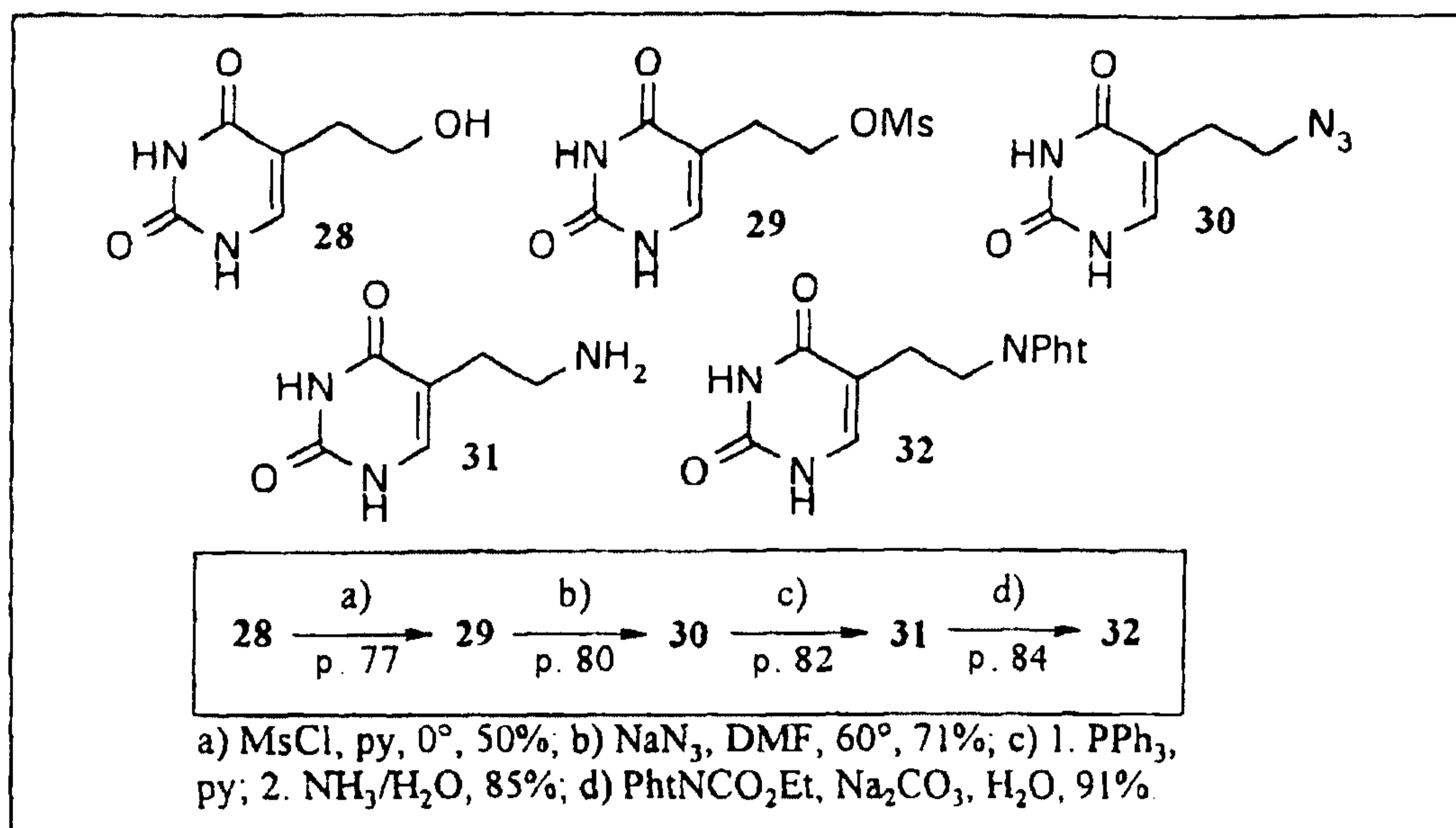
Scheme 5: Synthesis of N-phthaloylaminoethyluracil 32 .
