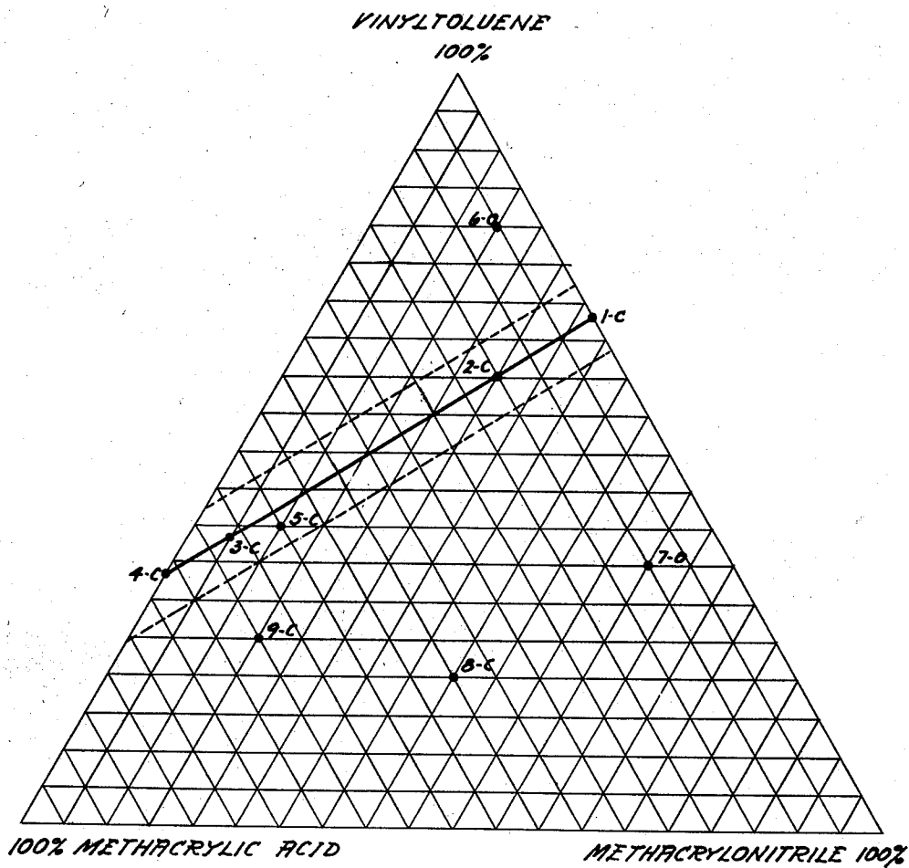
FIG. II. VINYLTOLUENE/METHACRYLIC ACID/METHACRYLONITRILE TERPOLYMERS WT. %
