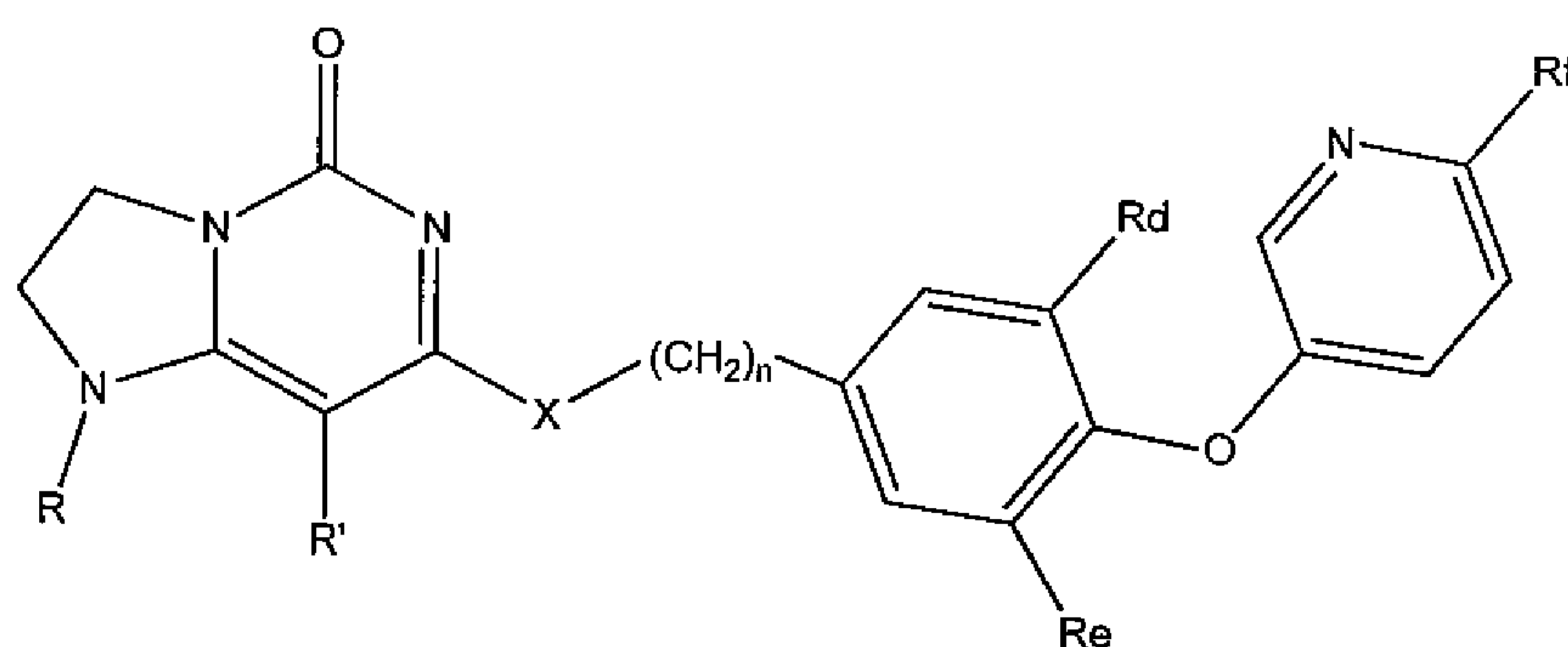
Formula (IB)
