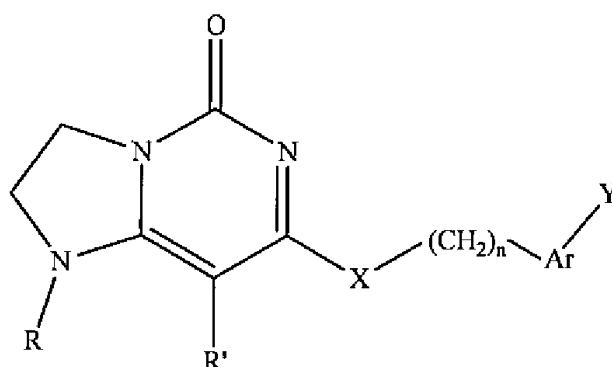
Formula (I)
