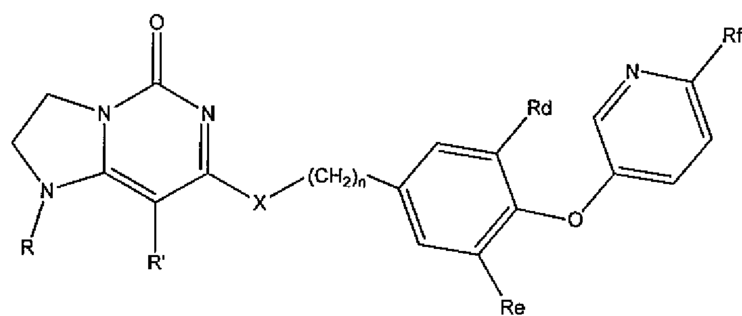
Formula (IB)
