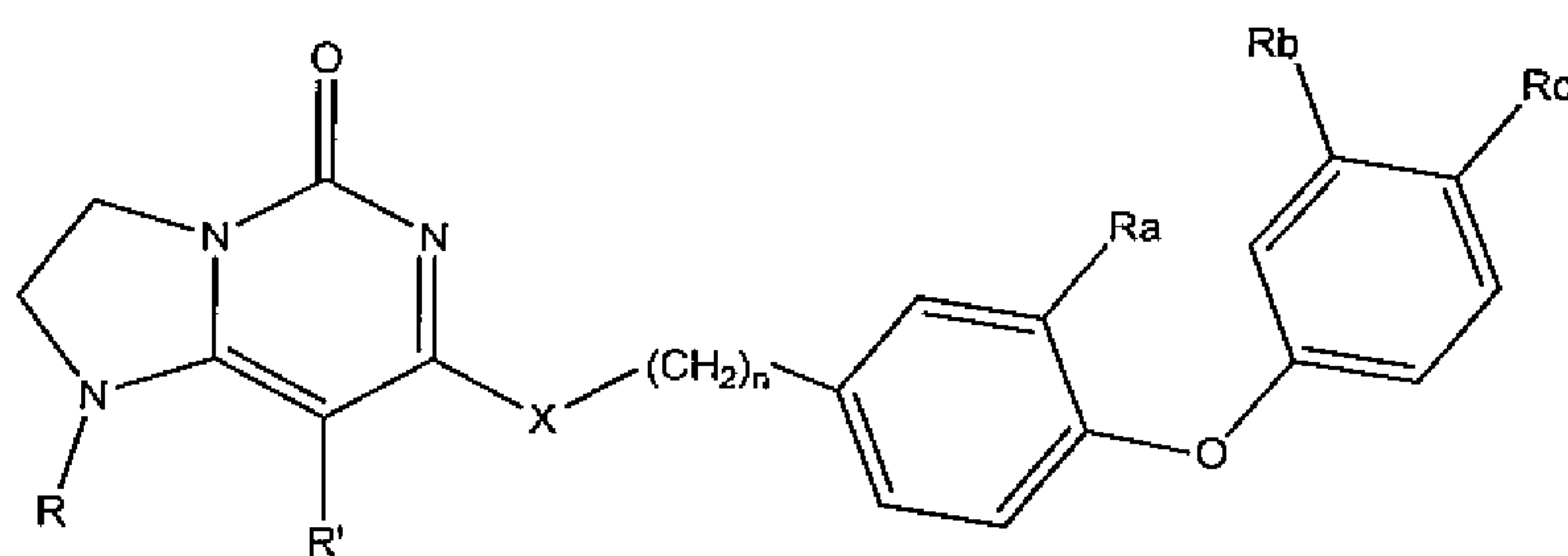
Formula (IA)
