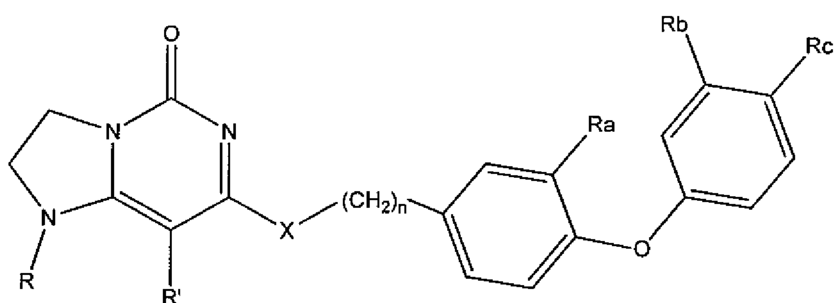
Formula (IA)
