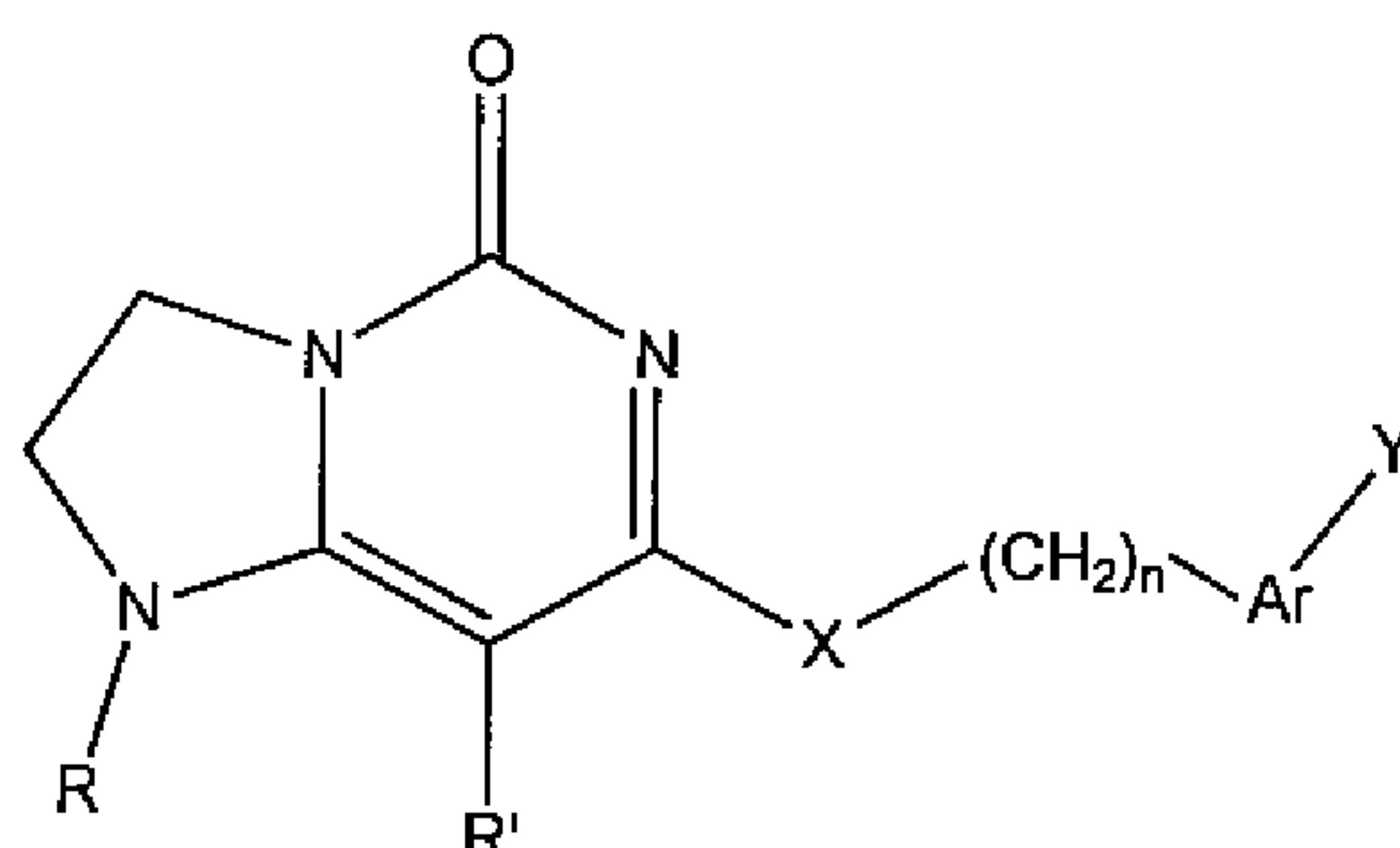
Formula (I)
