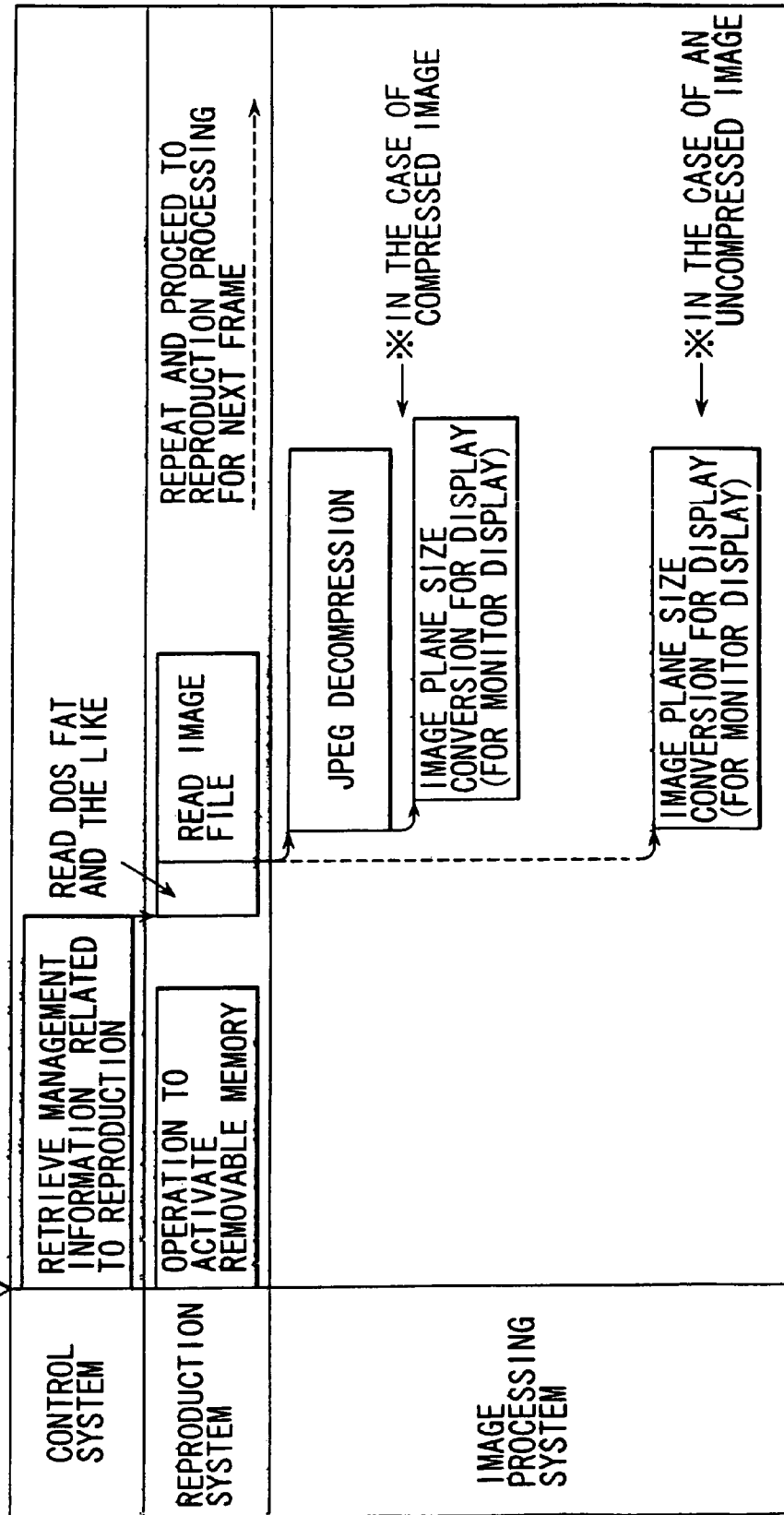
FIG. 5 OPERATING TIMING FOR REPRODUCTION REPRODUCTION MODE ON
