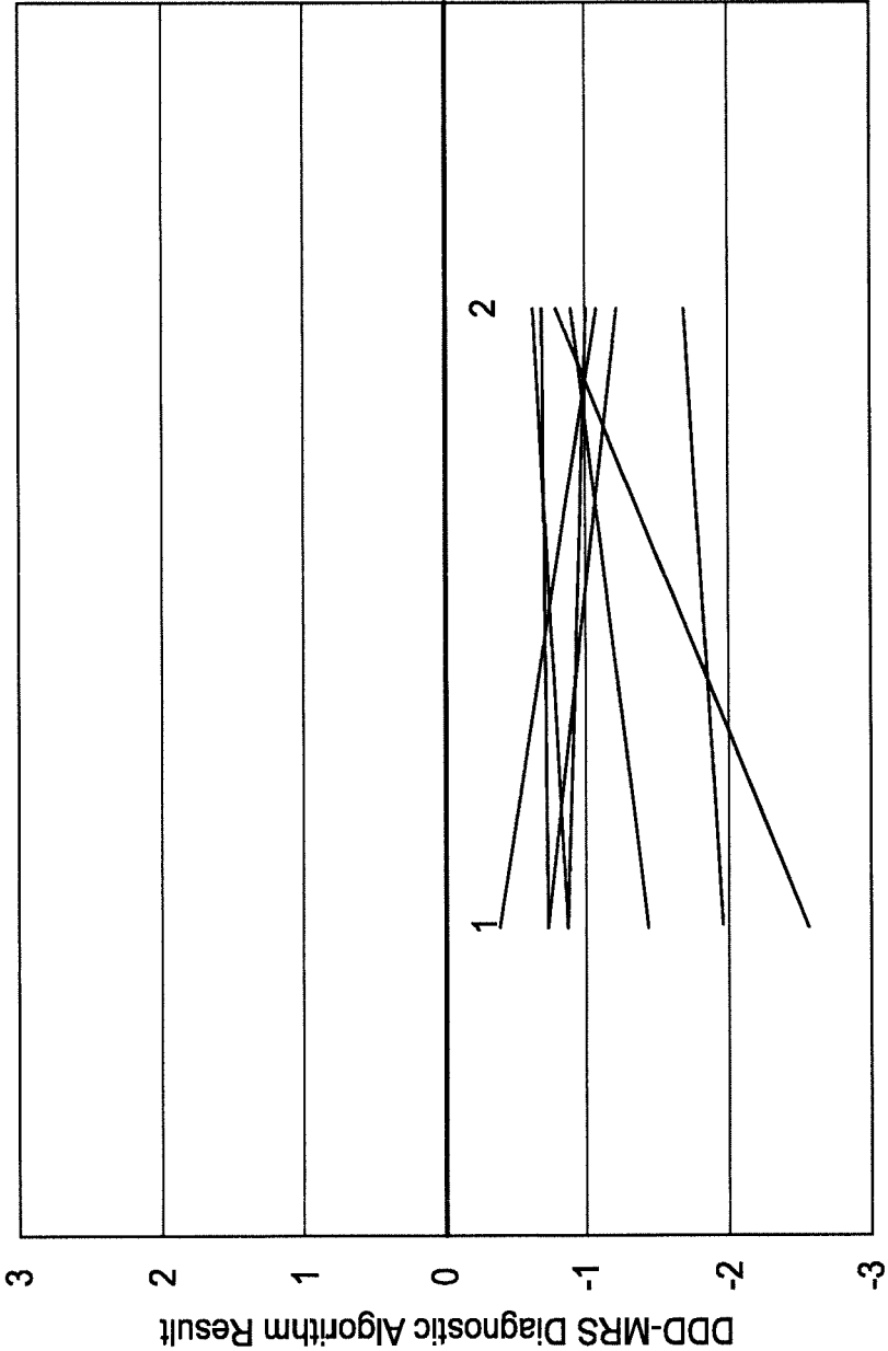
Separate DDD-MRS Acquisitions on Same Discs on Different Dates (n=8 L4L5 discs, Asymptomatic Control Volunteers)
