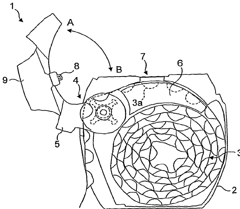
FIGURE 2 (PRIOR ART)
