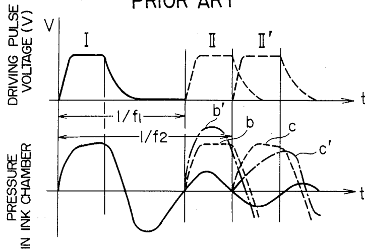
FIG. 4 PRIOR ART
