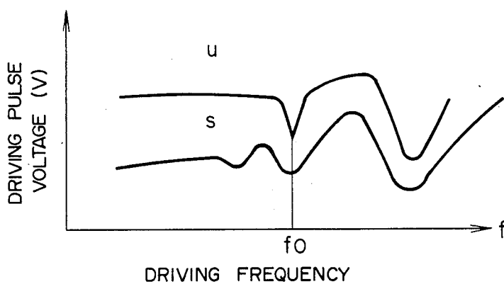
FIG. 3 PRIOR ART
