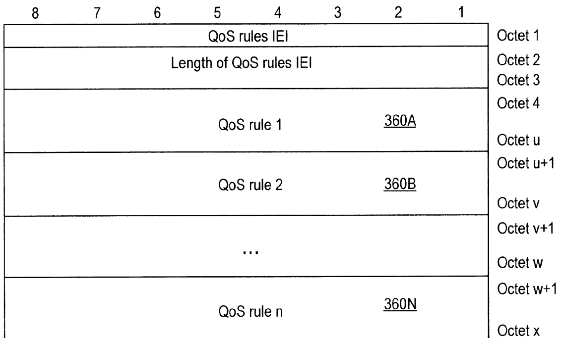
QoS rules information element
