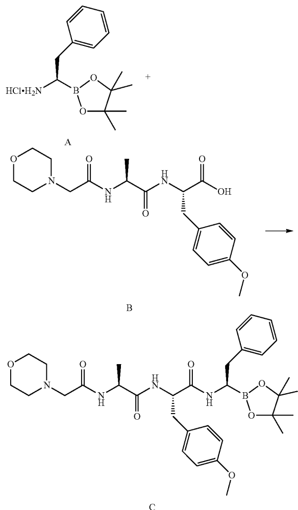
Scheme 1: Synthesis of Compound 1
